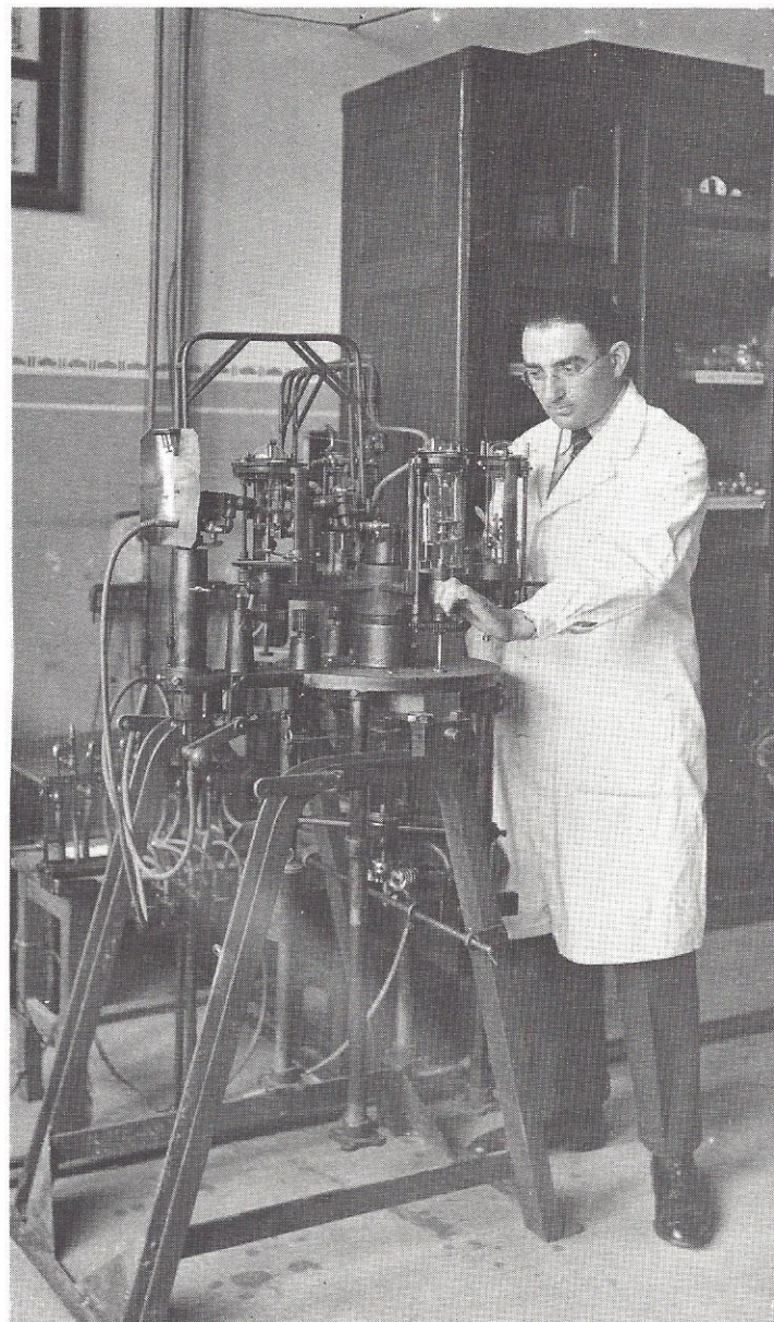
Figure 3b Bliss with the machine for sealing radio valves which he demonstrated before the Kammer Gericht Berlin, in his patent fight against Philips-Telefunken. (about 1933-1934)
